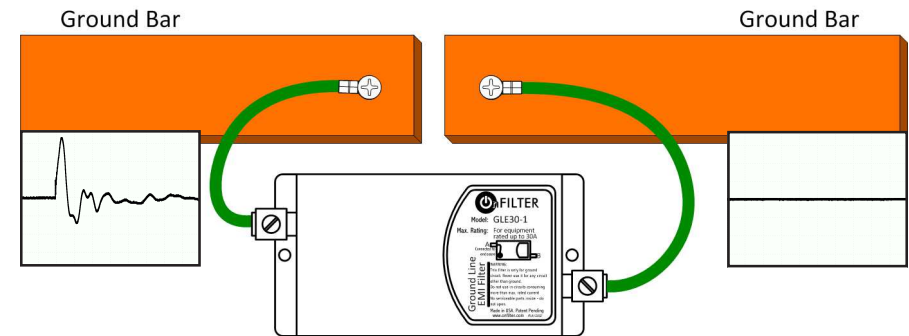
Example of Installation of OnFILTER' Ground Line Filter with Ground Bars
